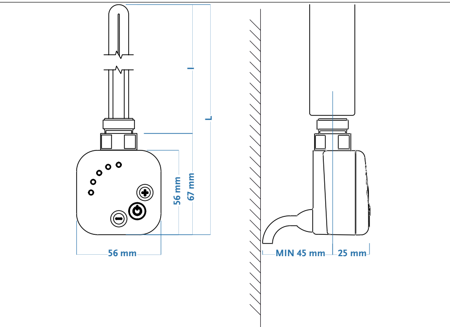
GK - schemat
